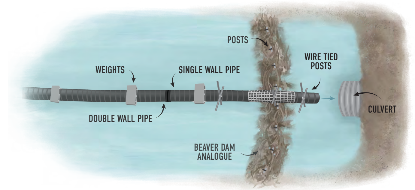
Figure 12. Combination of an anchor dam and pond leveler to create a pipe and dam culvert protection system.
