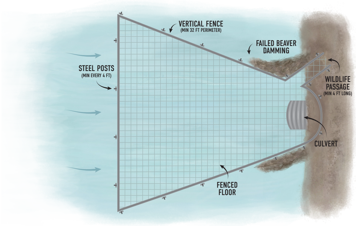
Figure 8. Trapezoidal culvert fence.
