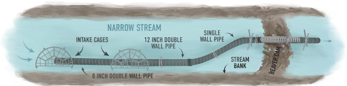
Figure 3. Overhead view of dual intake pond leveler modification for narrow streams using half-circle intake cages.
